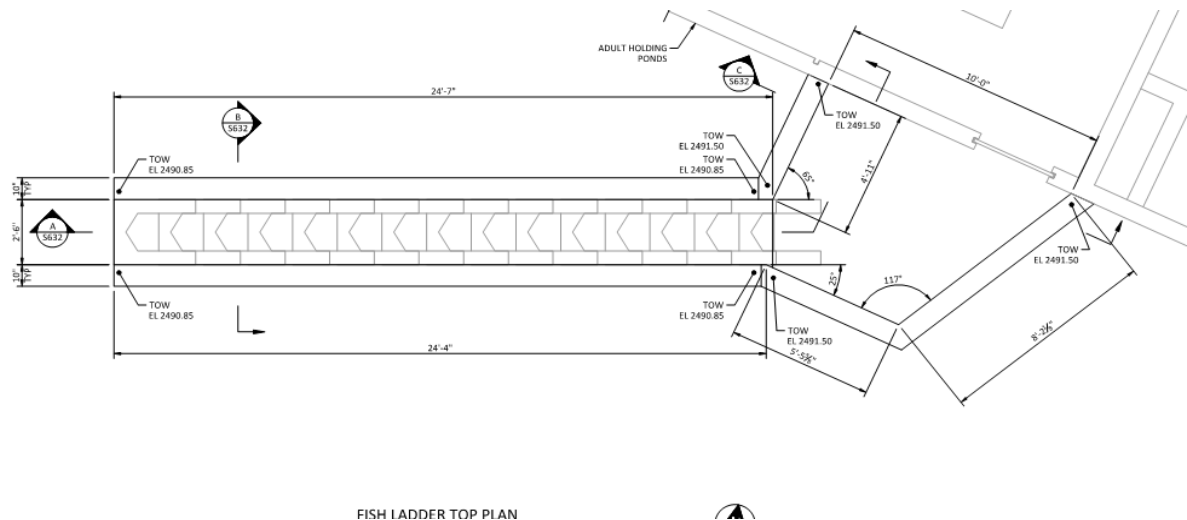
FISH LADDER TOP PLAN
