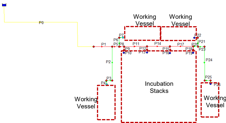
Figure 2. Pipe Naming Convention (Coho Building)
